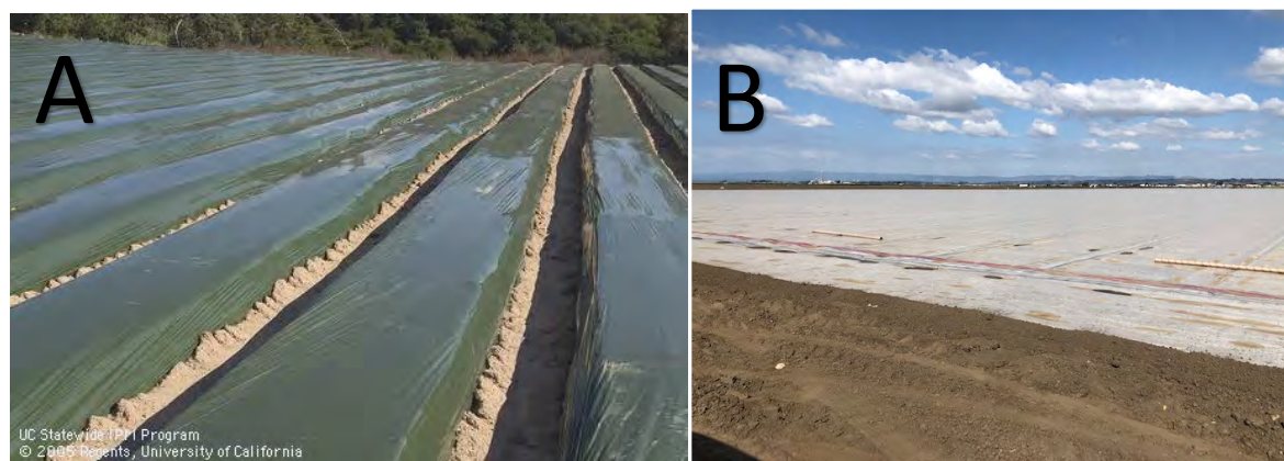
Figure 7. A) Beds are formed and covered with totally impermeable film (TIF) before drip fumigation. Furrows are not fumigated and pathogens can remain in the soil. B) Flat fumigation covers and treats the entire field, however uses twice the plastic because TIF fumigation film is removed and replaced with PE plastic mulch for bed formation. Photo credit: A) Jack Kelly Clark, B) Pam Krone
